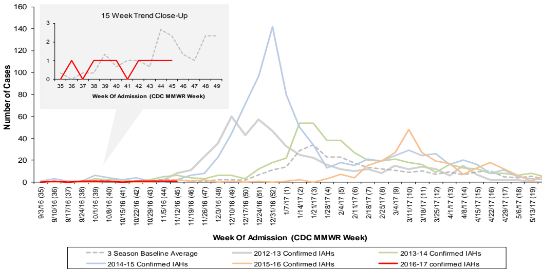
Figure 7: Franklin County Confirmed Influenza Associated Hospitalizations by Hospital Admission Week (As of 11/18/2016)
